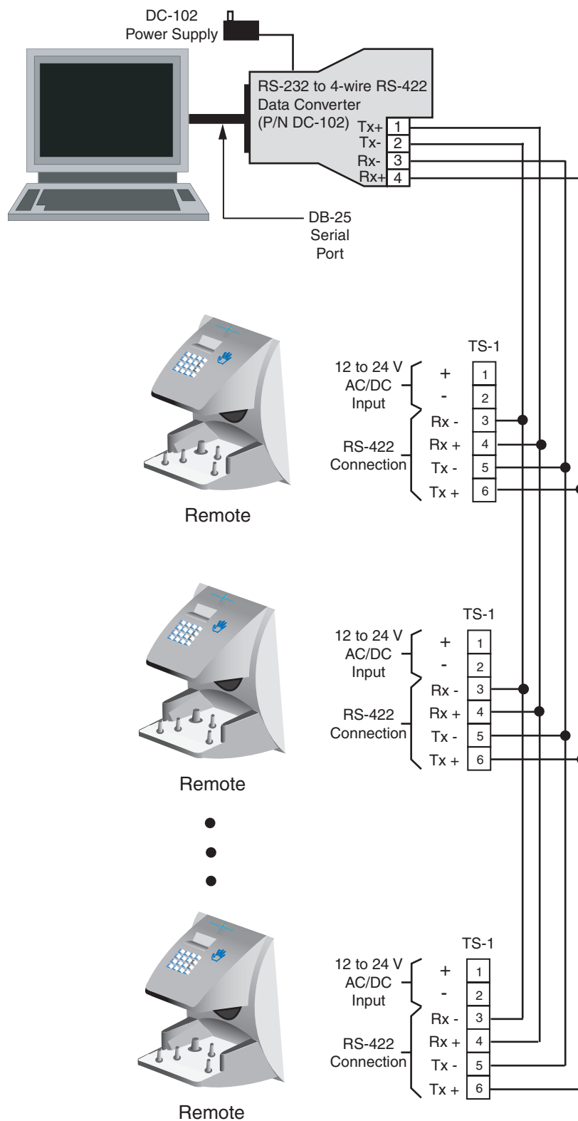
Figure 19-14: Host PC Network System Wiring Diagram
