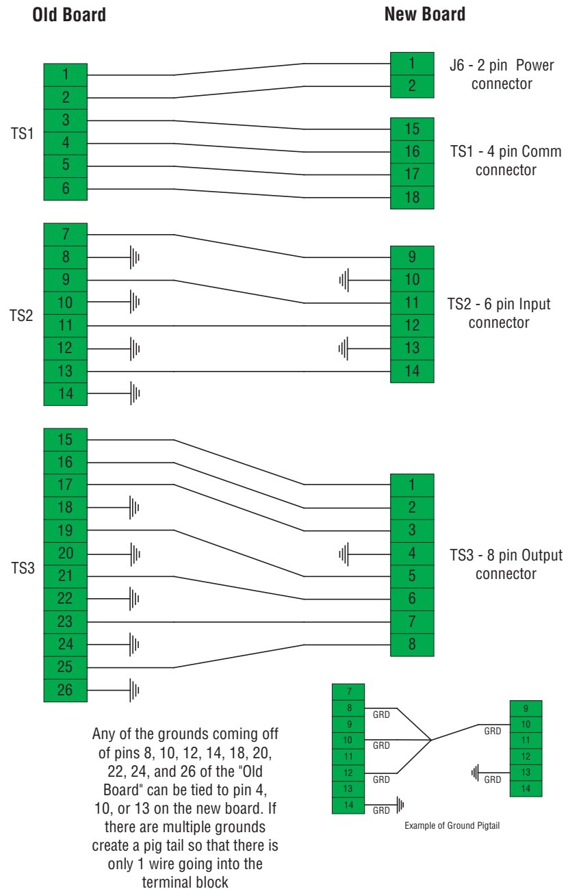
Figure 18-2: Terminal Block Layout
