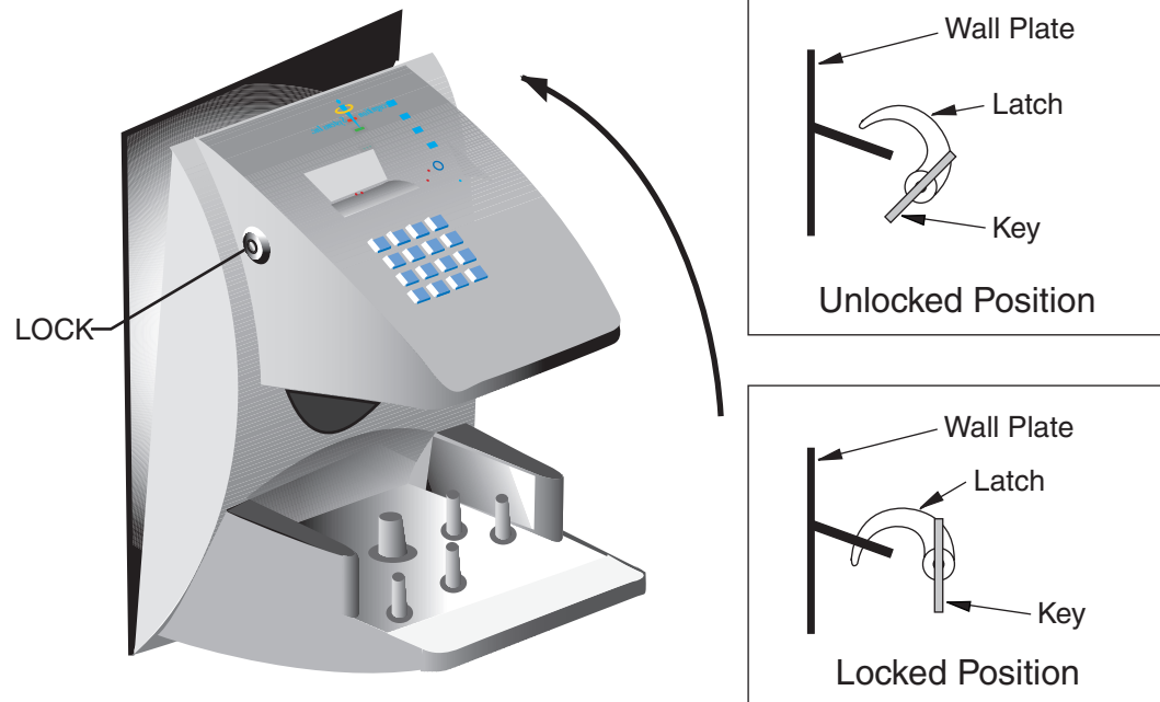
Figure 19-4: Closing the Hand Reader
